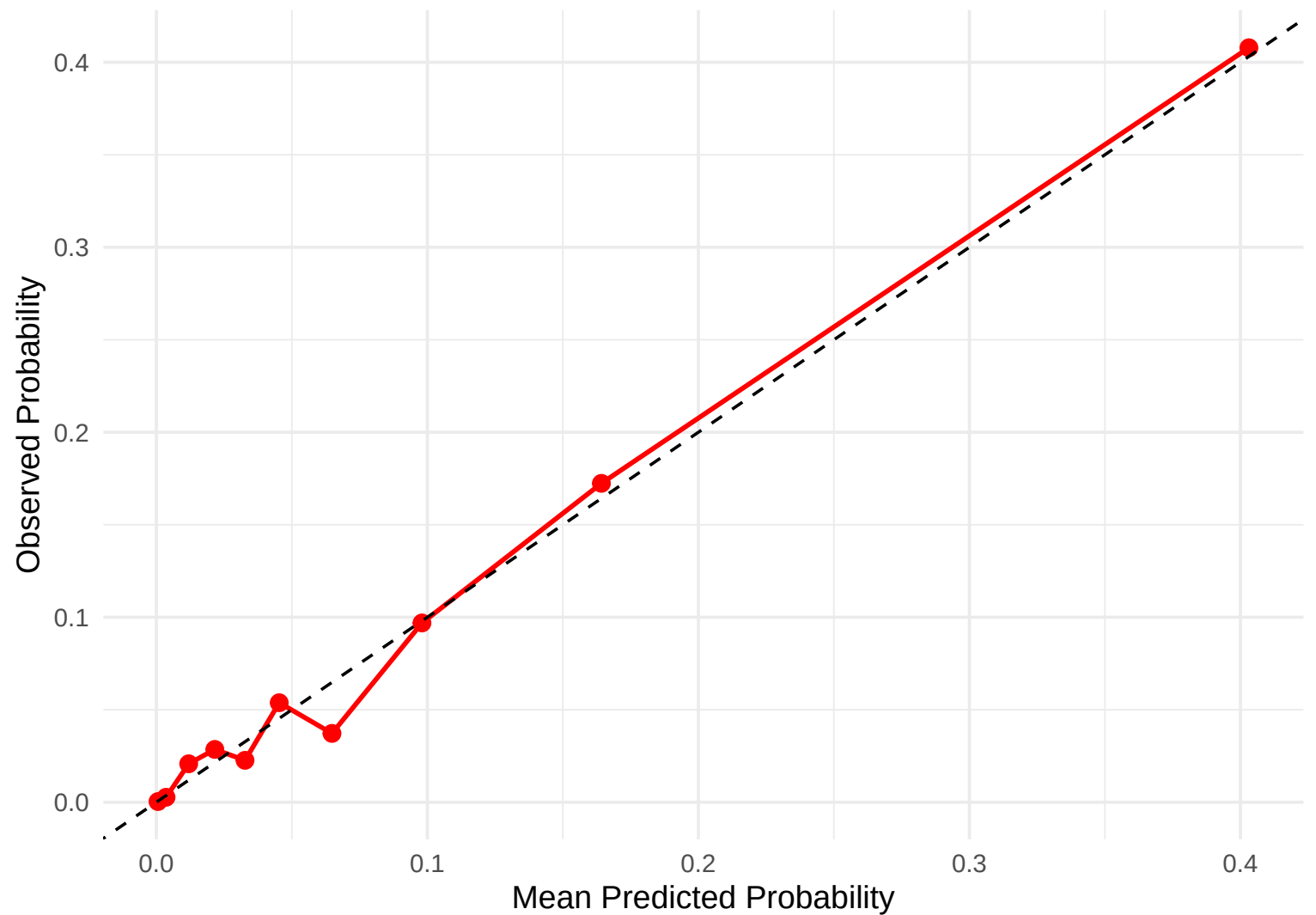
Calibration – cost_barrier
